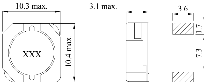
Land Pattern
